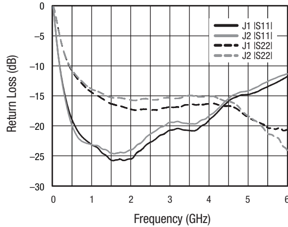
Figure 6. Return Loss vs Frequency (Isolation State)
