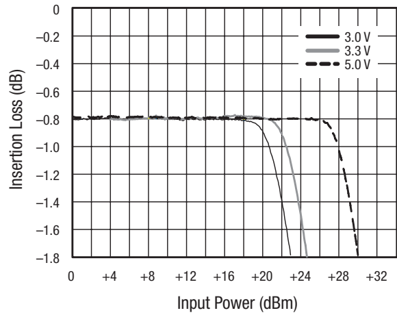
Figure 8. Insertion Loss vs Input Power Over Voltage
