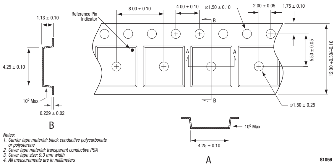
Figure 14. SKY13286-359LF Tape and Reel Dimensions
