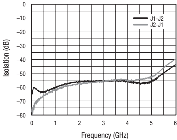
Figure 7. Output to Output Isolation
