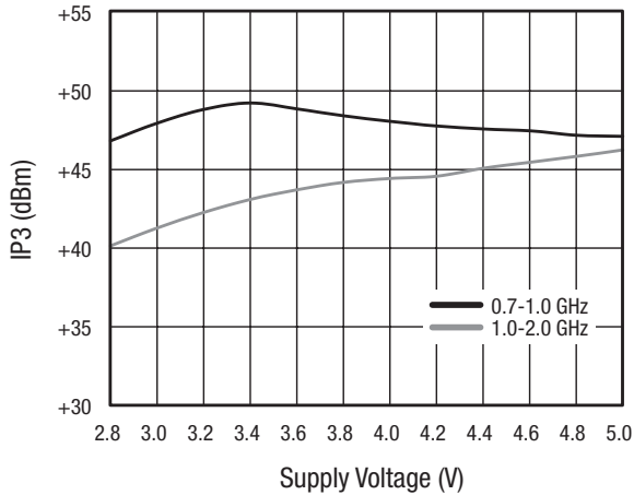
Figure 9. IP3 vs VDD Supply Voltage
